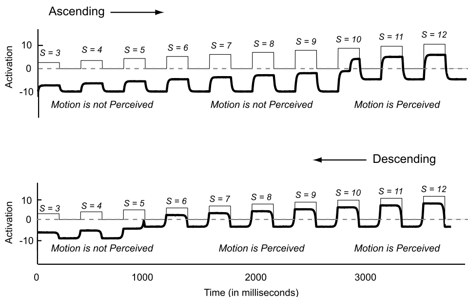
Figure 10. Simulation 4: single trial simulations for an ascending trial composed of a sequence of frames with increasing stimulus-initiated activation, and for a descending trial composed of a sequence of frames with decreasing stimulus-initiated activation. Hysteresis occurs when stimulus-initiated activation of the leftward or rightward detectors has crossed the self-excitation threshold of u = 0 and engages (ascending trials) or disengages (descending trials) the feedforward/feedback loop. It is indicated for end-point attribute values of S = 6, 7, 8 and 9 . Whether motion or nonmotion is perceived for these attribute values depends on the activational history that precedes their presentation i.e., motion is perceived when these attribute values are encountered during descending trials, and nonmotion is perceived when these attribute values are encountered during ascending trials. This is shown only for the leftward motion. The same result is obtained for rightward motion, which is not shown.
