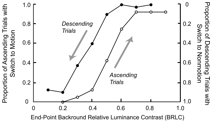
Figure 5. Hysteresis effect observed by gradually increasing or gradually decreasing the background relative luminance contrast (BRLC) for a participant in Hock et al. 's (1997) third experiment. The proportion of trials with switches from the perception of motion to the perception of nonmotion, and vice versa , are graphed as a function of the BRLC value at which each ascending or descending sequence of BRLC values ends. (Note the inversion of the axis on the right.)
