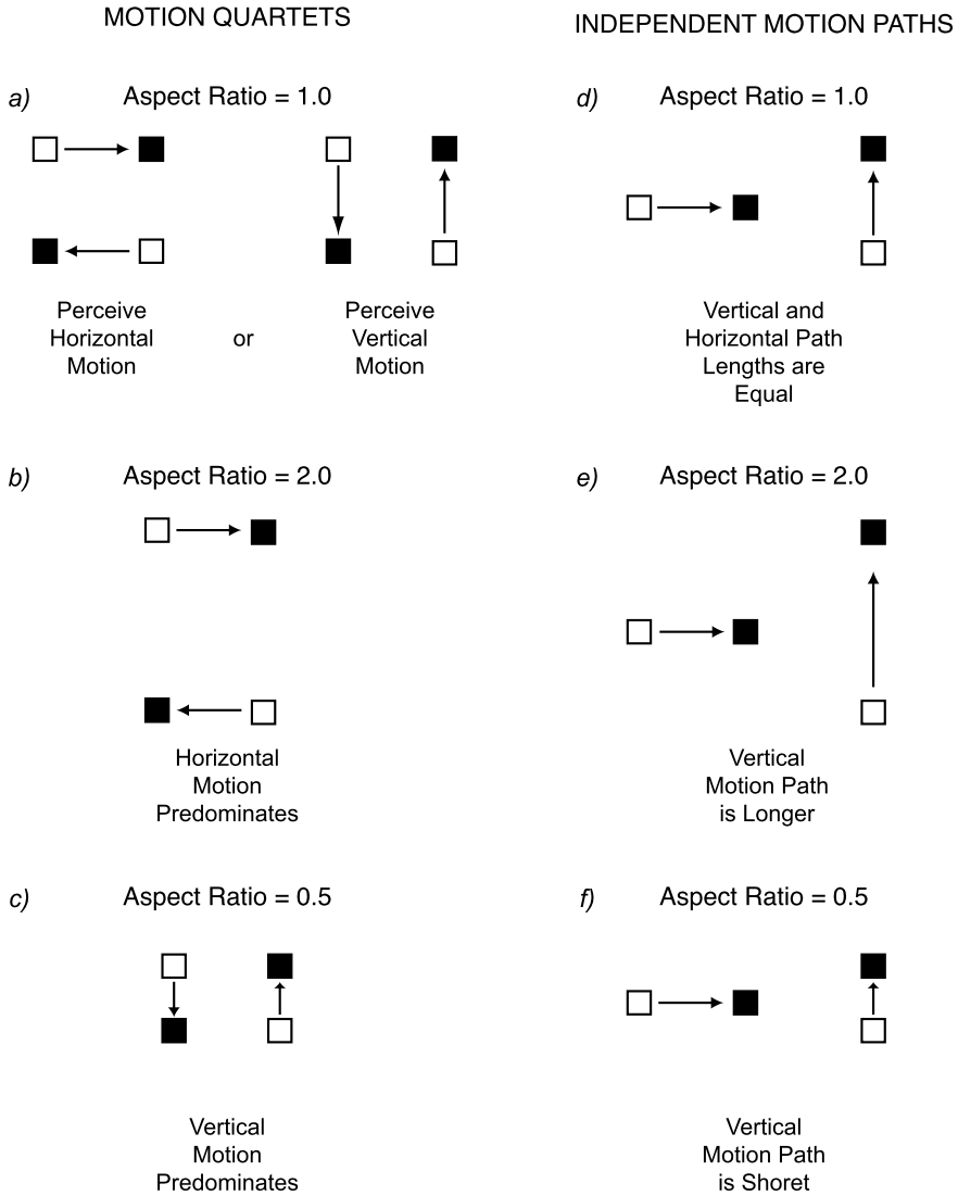
Figure 1. (a–c) Illustration of the motion quartets used in the hysteresis experiments reported by Hock et al. (1993) and Hock et al. (2005). Either parallel-path vertical motion or parallel-path horizontal motion is perceived, depending on the aspect ratio of the motion quartet (the vertical divided by the horizontal path length). (d–f) Stimuli with independent vertical and horizontal motions that were matched in aspect ratio with the motion quartets in Hock et al. (2005).
