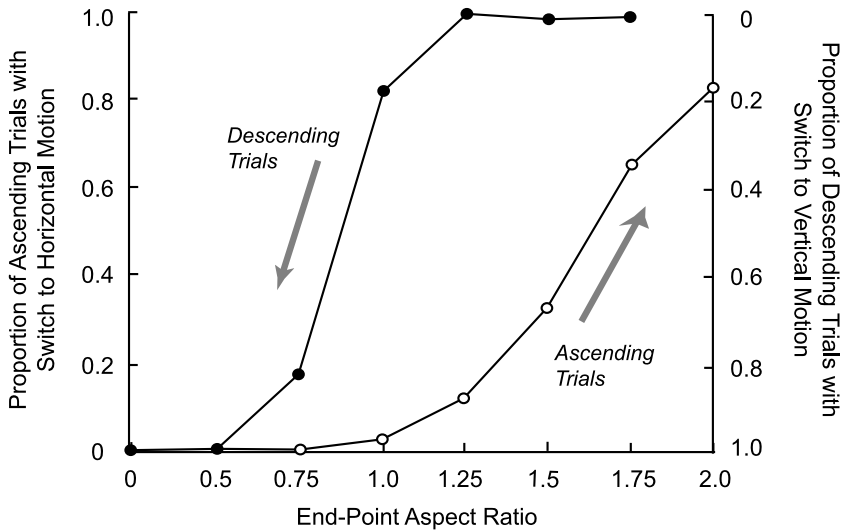
Figure 2. Hysteresis effect observed by gradually increasing or gradually decreasing the aspect ratio of a motion quartet for a participant in Hock et al. 's (1993) second experiment. The proportion of trials with switches from horizontal to vertical motion, and vice versa , are graphed as a function of the aspect ratio at which each ascending or descending sequence of aspect ratios ends. (Note the inversion of the axis on the right.)
