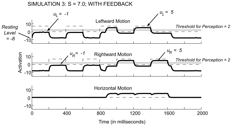
Figure 9. Simulation 3: single trial simulation for stimulus-initiated activation ( S = 7.0 ) that would be insufficient to engage the feedforward/feedback loop (as was the case during the first part of the simulated trial) were it not for random fluctuations in activation that crossed the self-excitation threshold for a detection instability (as occurred during the second part of the simulated trial).
