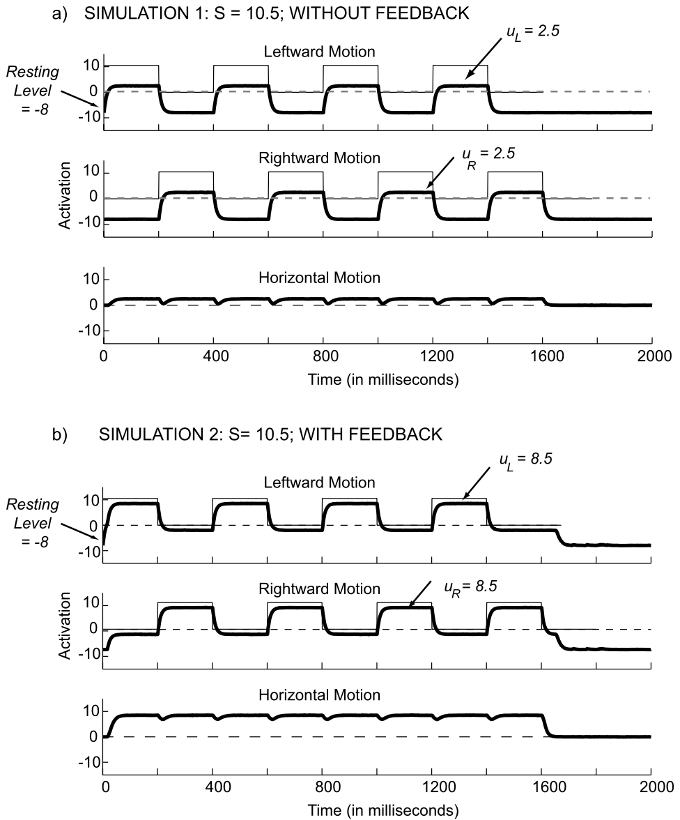
Figure 8. (a) Simulation 1: single trial simulation without feedback for stimulus-initiated activation ( S = 10.5 ) that just exceeds the read-out threshold ( u = 2 ), which determines whether there is sufficient detector activation to signal the perception of motion. (b) Simulation 2: single trial simulation for the same stimulus, but with feedback from the bidirectional horizontal motion detector boosting the activation of the unidirectional leftward or rightward motion detectors. This occurs when the stimulus-initiated activation of the leftward or rightward detectors is sufficient for activation to pass through a detection instability (the feedforward/feedback loop is engaged when the activation of the leftward or rightward detector exceeds the threshold for self-excitation ( u = 0 in these simulations)).
