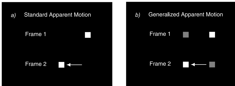
Figure 4. Examples of standard and generalized apparent motion stimuli.
