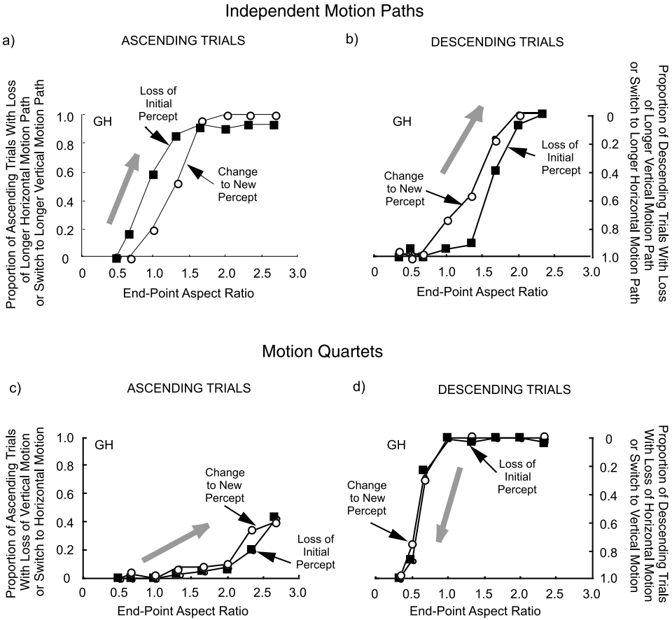
Figure 3. Results for one of the participants in Hock et al. 's (2005) comparison of hysteresis effects for motion quartets and for stimuli with independent vertical and horizontal motion paths. In separate blocks of trials, the participants reported whether or not they 'lost' their initial percept anytime during a trial, or whether or not there was a change to the alternative percept anytime during a trial. The results for these response criteria are reported separately for trials with ascending and trials with descending aspect ratios, for both independent motion paths, (a) and (b), and for motion quartets (c) and (d).
