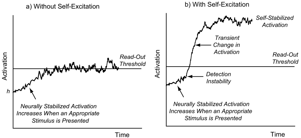
Figure 6. Illustration of detector activation increasing from its no-stimulus resting level ( h ) upon the presentation of a stimulus attribute to which it responds. The increasing activation is stabilized by intrinsic neural mechanisms. Panel (a) illustrates why perception would be unstable if the steady-state activation value were near the read-out threshold for the detector, which determines whether or not there is sufficient activation for the stimulus attribute to be perceived. Panel (b) illustrates the transient increase in detector activation (i.e., the detection instability) that would result from activation crossing a self-excitation threshold, with activation stabilizing at a level that is well above the read-out threshold.
