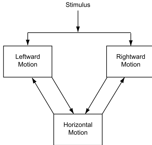
Figure 7. A feedforward/feedback model implementing detection instability. It is composed of unidirectional leftward and rightward motion detectors whose stimulus-initiated activation, if greater than 0, feeds forward to a bidirectional horizontal motion detector. Excitatory feedback from the horizontal to the leftward and rightward detectors boosts their activation.
